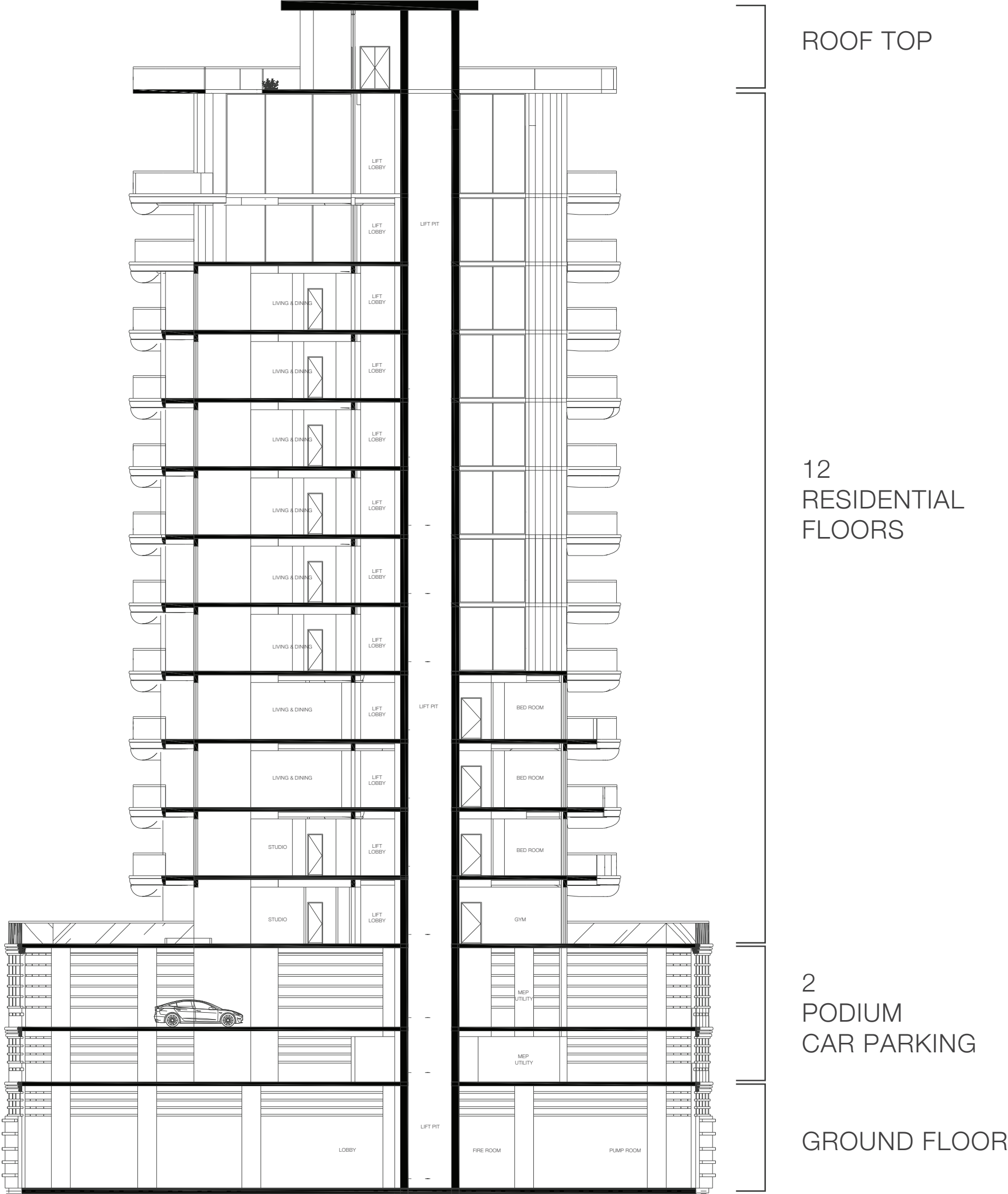
G + 2 PODIUM CAR PARKING + 12 RESIDENTIAL FLOORS
